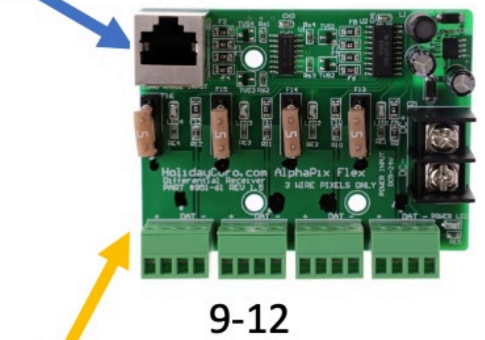
4 Port LR Dumb Receiver
